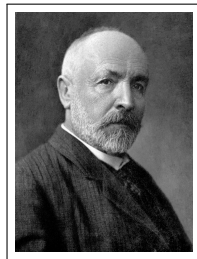
Georg Cantor (1845 – 1918)
